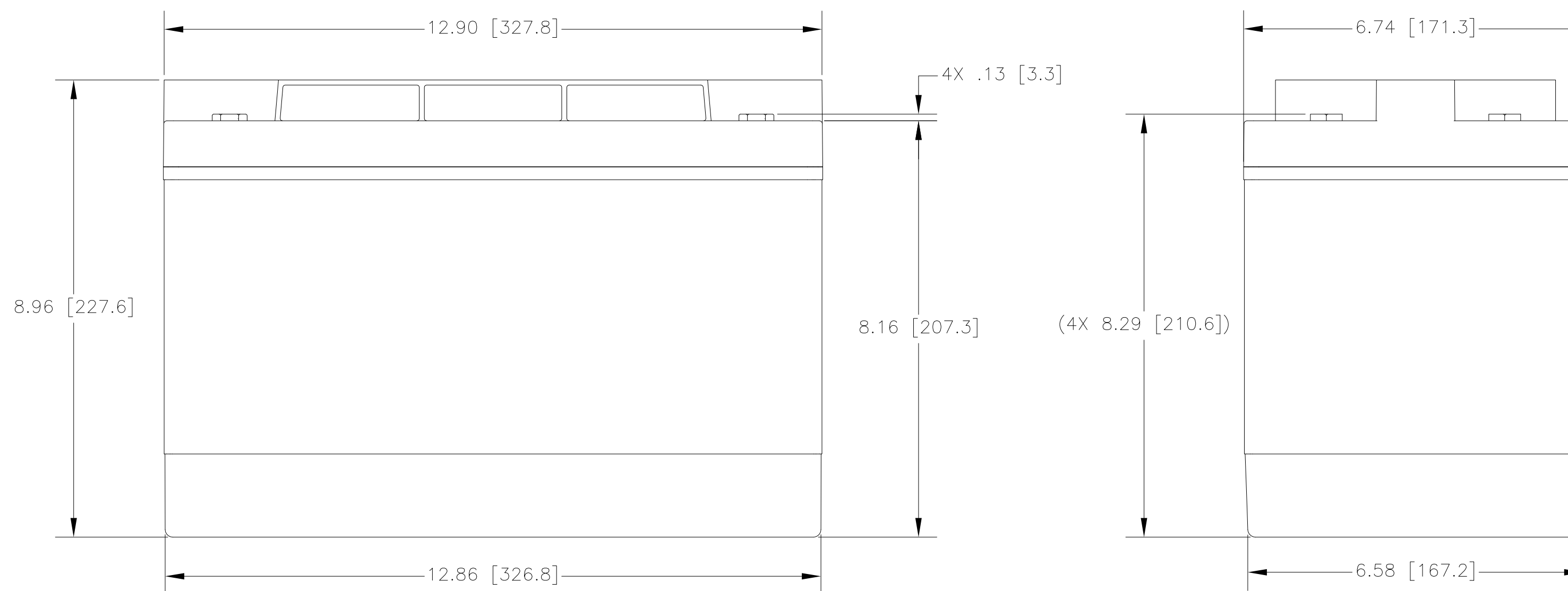
ENVELOPE DRAWING
